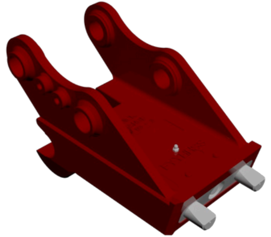
Quick Coupler CNC03 Mechanic
